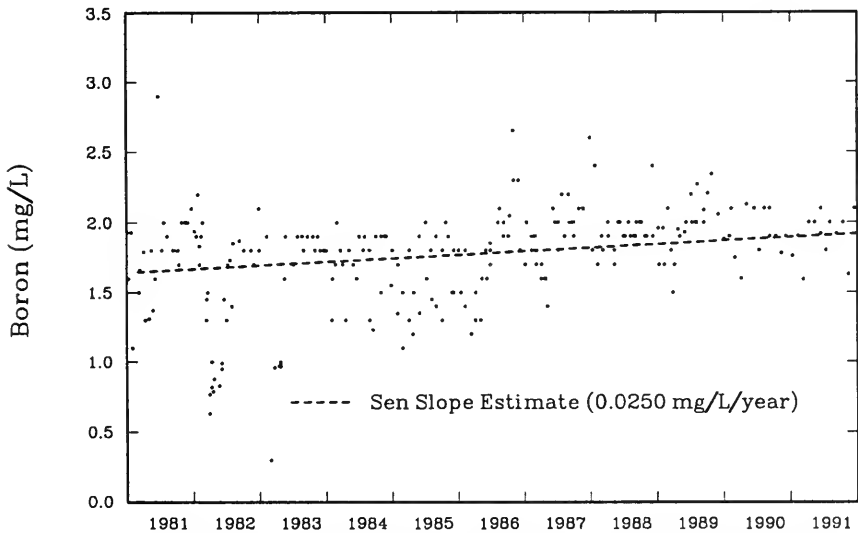
Figure 3.10 Sen Slope Estimate for Boron at East Poplar River at the International Boundary.
